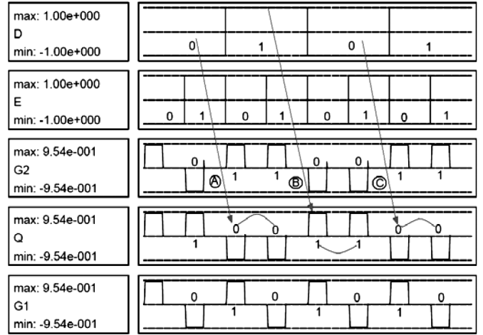
Fig. 11. Simulation of D latch with output Q .
