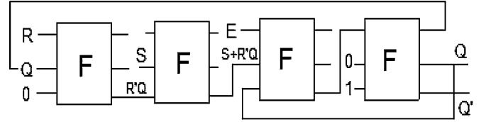
Fig. 8. Concurrently testable SR latch design.
