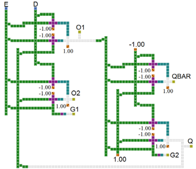
Fig. 12. QCA layout of D latch with output Q as well as complement output QBAR .
